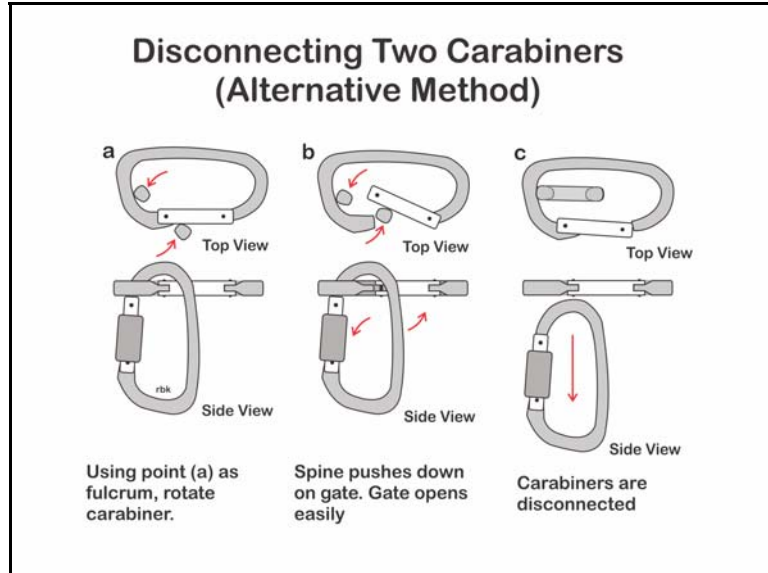
Figure 30: Disconnecting Two Carabiners (Alternative Approach). In swiftwater situations, two carabiners can easily become disconnected. Source: Author.
