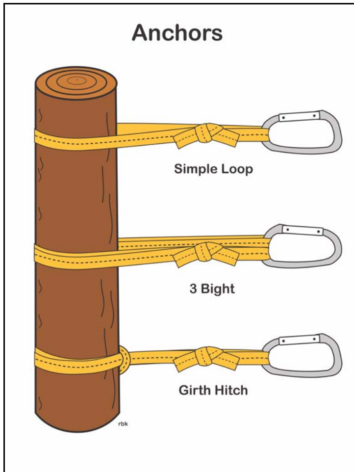
Figure 27: Three Examples of Anchors. Source: author.
