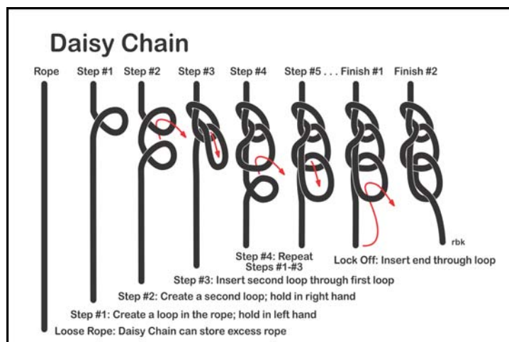
Figure 7: Daisy Chain. The Daisy Chain is a method of temporarily storing excess rope. Source: Author.
